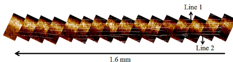
Figure 3. Representative AFM image of complete DNA spokes with a total length of 1.6 mm formed at \text{pH} = 6.2 , T = 65^\circ\text{C} , and the concentration of DNA solution = 8\ \mu\text{g/mL} . The arrow marked the direction of drying front during the course of water evaporation. The cross-sectional analysis of Line 1 and Line 2 is summarized in Figure S1.
